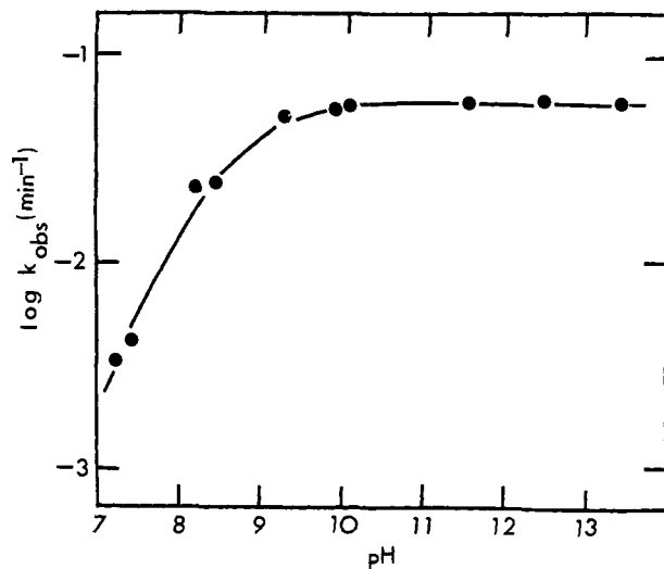
Figure 2. The pH-log k_{\text{obsd}} profile for the hydrolysis of 1-methyl-5-difluoromethyluracil (6) at 30°.
