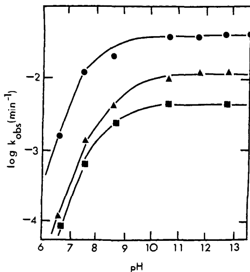
Figure 1. The pH-log k_{\text{obsd}} profiles for the hydrolyses of 1 (▲), 2 (●), and 3 (■) at 30°.
