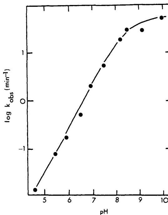
Figure 3. The partial pH-log k_{\text{obsd}} profile for the hydrolysis of 5-difluoromethyluracil (5) at 30°.
