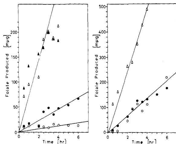
Figure 5. Kinetics of inhibition of folate synthesis by N 1 -4-nitrophenylsulfonamide with and without preincubation. (a, left) Kinetics of inhibition where the sulfonamide (12 \mu M) and 7,8-dihydro-6-hydroxymethylpterin (32 \mu M) were preincubated for 3 hr and PABA (20 \mu M) was subsequently added (○○○) and where sulfonamide (12 \mu M), pterin component (32 \mu M), and PABA (20 \mu M) were added together to the reaction mixture at zero time (●●●). The appropriate controls where no sulfonamide was added are \Delta\Delta\Delta and \blacktriangle\blacktriangle\blacktriangle . (b, right) Kinetics of inhibition by N 1 -4-nitrophenylsulfonamide as under (a); however, the concentration of 7,8-dihydro-6-hydroxymethylpterin was 54 \mu M (○○○ and ●●●, control \Delta\Delta\Delta ).
