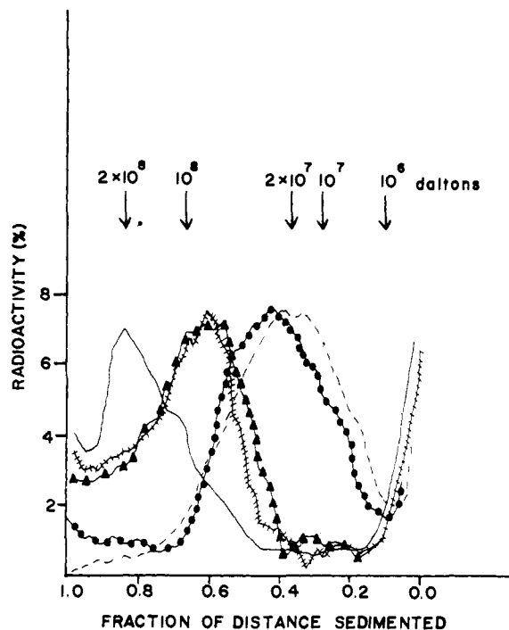
Figure 3. Sedimentation profiles for isolated DNA treated at 10 krad in the presence or absence of 5 mM analog. (—) no analog, 0 krad; (---) no analog, 10 krad; (+++++) trans -3 + 10 krad; (—▲—▲—▲) MEA (1) + 10 krad; (—●—●—●) cis -3 + 10 krad. Sedimentation profiles were obtained by centrifugation at 35,000 rpm for 180 min on a 4-ml gradient containing 5-20% alkaline sucrose with a 0.2-ml 60% sucrose cushion layer and a 0.2-ml alkaline overlay.
