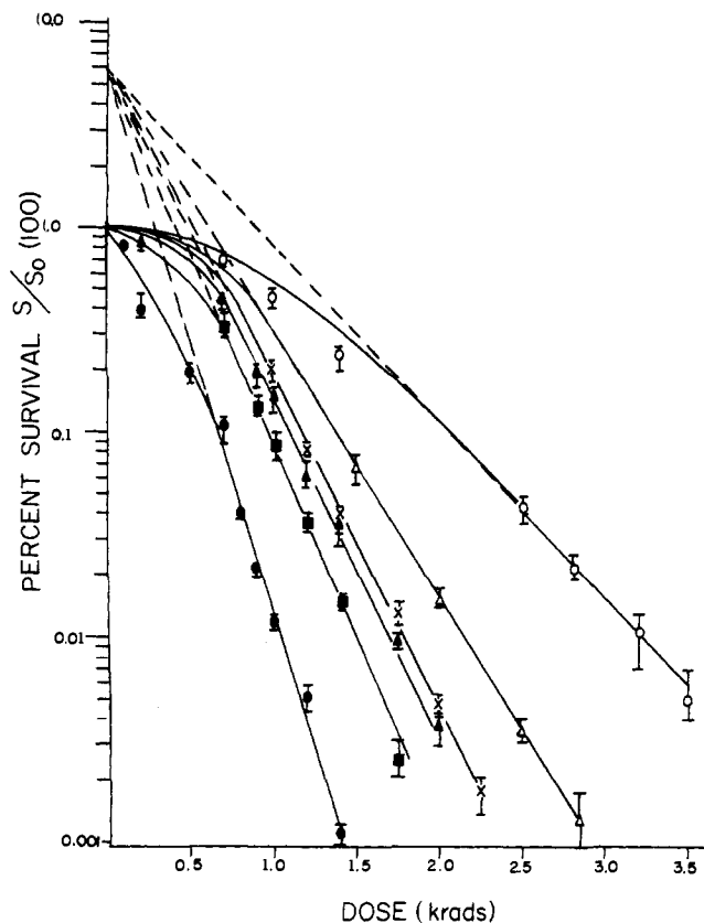
Figure 2. Dose-survival curves for Chinese hamster cells irradiated under aerobic conditions in the presence or absence of various analogs (5.0 mM). (—○—○—○) no analog, cells under N 2 ; (—Δ—Δ—Δ) trans -3; (—×—×—×) trans -2; (—▲—▲—▲) MEA (1); (—■—■—■) trans -4; (—●—●—●) no analog, cells under air.
