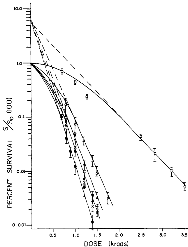
Figure 1. Dose-survival curves for Chinese hamster cells irradiated under aerobic conditions in the presence or absence of various analogs (2.5 mM). (—○—○—○) no analog, cells under N 2 ; (—Δ—Δ—Δ) trans -3 (points shown), trans -4 (points not shown), no significant difference between trans -3 and trans -4; (—▲—▲—▲) MEA (1) (points shown), or trans -2 (points not shown), no significant difference between 1 and trans -2; (—×—×—× and —■—■—■) cis -3 and cis -2, respectively, no significant difference; (—●—●—●) no analog, cells under air.
