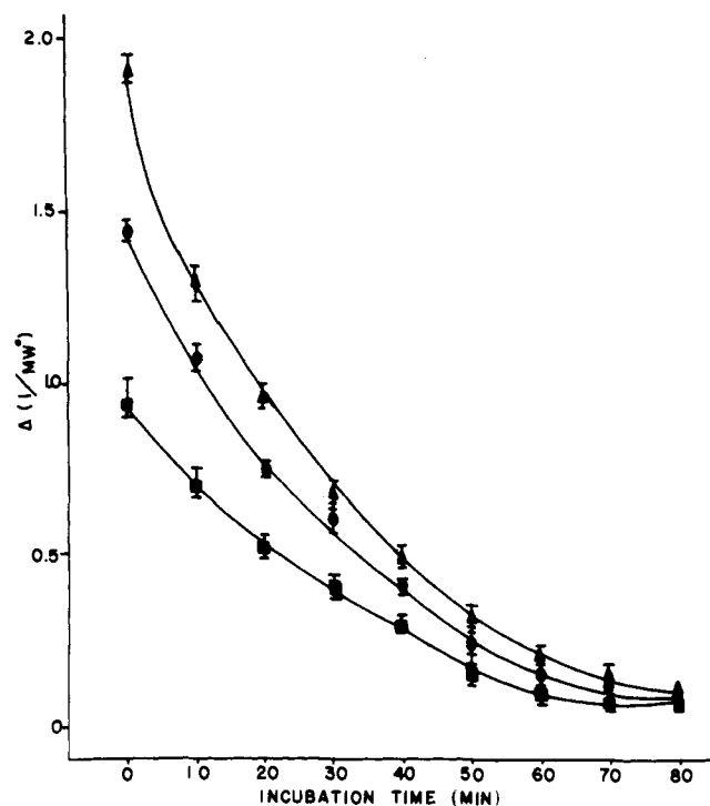
Figure 5. Rejoining of single strand breaks in DNA induced by 20 krad \gamma irradiation followed by incubation at 37° for varying times. (— \Delta — \Delta — \Delta —) absence of mercaptoalkylamines; (— \bullet — \bullet — \bullet —) 5 mM cis -3; (— \blacksquare — \blacksquare — \blacksquare —) 5 mM trans -3.
