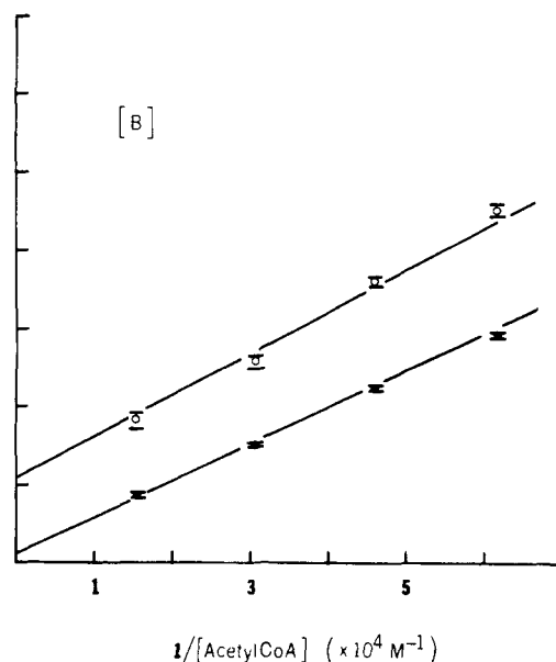
Figure 3. Kinetics of ChAc inhibition by acryl-DMA: (●) control; (○) acryl-DMA. [A] acryl-DMA, 0.2 mM; choline, 0.4-4.0 mM; acetyl-CoA, 0.65 mM. [B] acryl-DMA, 1.0 mM; choline, 25 mM; acetyl-CoA, 0.016-0.065 mM. Each point is a mean of three experiments and bars represent SEM.
