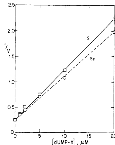
Figure 2. Dixon plots of the kinetics of inhibition of L. casei thymidylate synthetase by IV (O, X = Se) and 5-mercapto-2'-deoxyuridylic acid (□, X = S). Substrate concentration used: 2.5 \times 10^{-4} M; v = \Delta\text{OD}_{340}/\text{min} .
