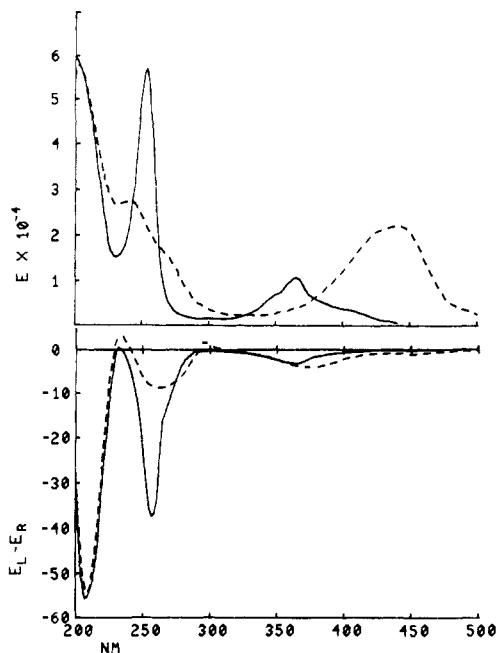
Figure 1. Absorption (top) and circular dichroism (bottom) spectra in 0.01 M phosphate buffer (pH 7) containing EDTA, 10^{-5} M; actinomycin D (---), 3 \times 10^{-5} M; and 2 (—), 3 \times 10^{-6} M.
