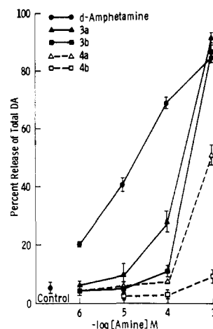
Figure 3. Release of [ 3 H]dopamine from isolated corpus striatum by amphetamine and rigid analogues of amphetamine. See legend to Figure 2 for design of experiment. Each value represents the mean ± SEM of three to four values. Control represents release in samples which were incubated in the absence of drug.
