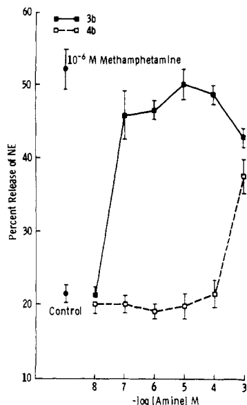
Figure 8. The effect of methamphetamine and the rigid analogues on the release of previously accumulated L - ^3\text{H} NE from reserpine- and pargyline-treated rat atrial tissue. Tissue which had previously accumulated the ^3\text{H} -labeled amine was incubated for 15 min with various concentrations of the drugs. Release of ^3\text{H} norepinephrine is expressed as a percentage of the total ^3\text{H} -labeled amine (medium + tissue). Each value is the mean \pm SEM of three to six experiments. Control represents release in samples which were incubated in the absence of drug. Dose-response curves for methamphetamine are reproducible in these assays, so the value at only 10^{-6} M is given here. See ref 2 for the complete dose-response curve for methamphetamine.
