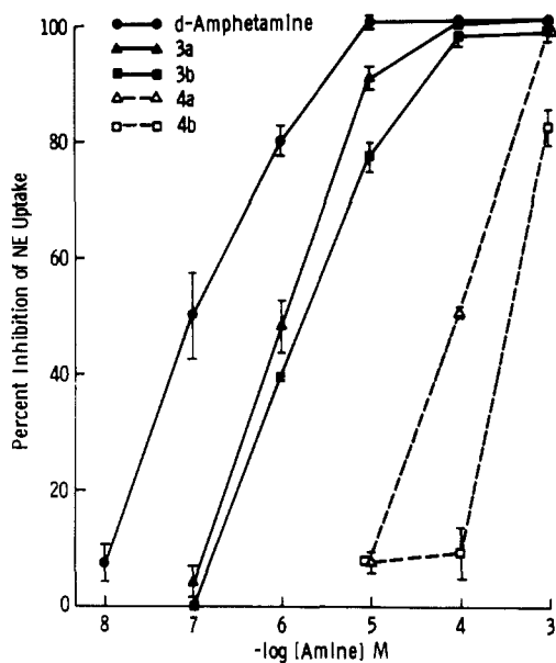
Figure 1. Inhibition of uptake of [ 3 H]norepinephrine into cerebral cortex tissue by amphetamine and rigid analogues of amphetamine. Chopped cerebral cortex was incubated for 10 min with various concentrations (10 -8 to 10 -3 M) of the compounds. [ 3 H]Norepinephrine (10 -7 M) was then added, and the incubation was continued an additional 10 min. Tritium was measured in tissue and medium. Inhibition of neuronal uptake is expressed as a percentage of control values (mean ± SEM) for three to four experiments. The mean tissue/medium ratio for uptake in control samples was 7.1 ± 0.4.
