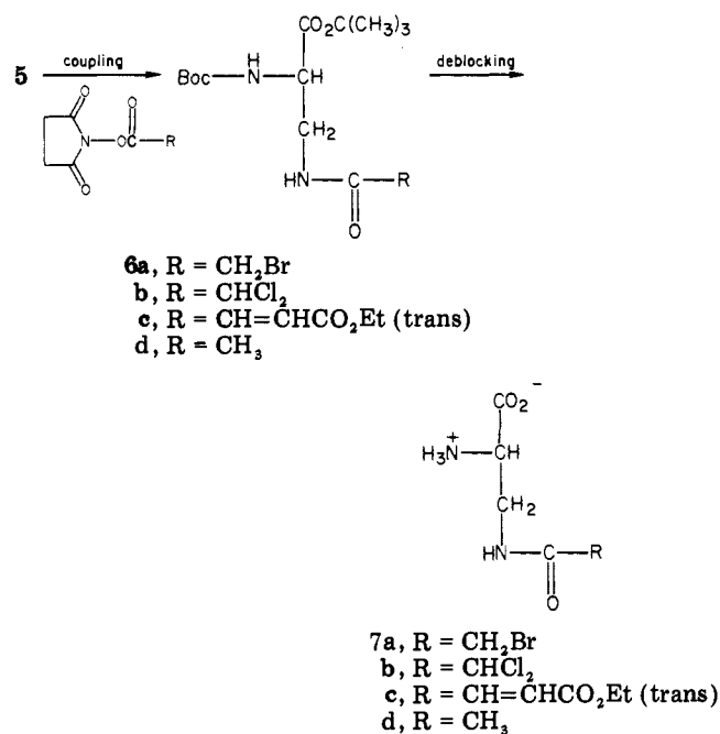
Scheme II a
