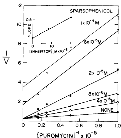
Figure 1. Lineweaver-Burk plot of the effect of sparsophenicol ( 1b ) on the rate of N -acetyl-L-[ 14 C]phenylalanylpuromycin formation. Inset shows the linear relationship between the slope and inhibitor concentration in the concentration range where the inhibition was competitive. The complex of N -acetyl-L-[ 14 C]-phenylalanyl tRNA-70S E. coli ribosome-poly(U) was employed in the reaction with puromycin as specified in ref 1.
