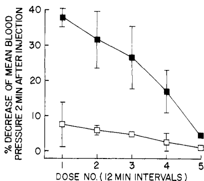
Figure 3. Effects of 3 and 4 on mean blood pressure 2 min after injection: (■) 3 (15 \mu\text{mol}/\text{kg} ) ( n = 3 ); (□) 4 (15 \mu\text{mol}/\text{kg} ) ( n = 3 ). Results are expressed as the mean \pm SEM.
