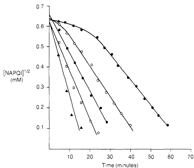
Figure 1. Decomposition rate plots for 0.4 mM NAPQI in 0.1 M sodium phosphate buffer, pH 7.4: NAPQI alone (●) and with inclusion of 8 (○), 20 (■), 40 (□), and 80 \mu M (▲) acetaminophen.
