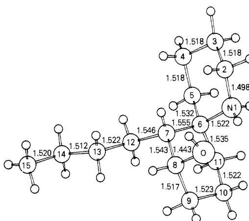
Figure 1. X-ray structure and bond lengths for (±)-2-depentylperhydrohistrionicotoxin hydrobromide (4·HBr). ESDS of bond length is <0.006 Å.
