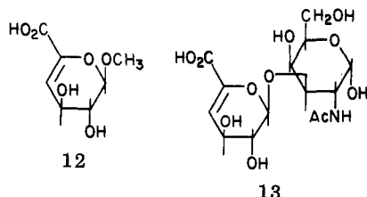
L -threo-hex-4-enopyranosiduronic acid)-(1 \rightarrow 3)-2-acetamido-2-deoxy- \alpha -D-galactopyranose 19 ( 13 ), the double bonds
