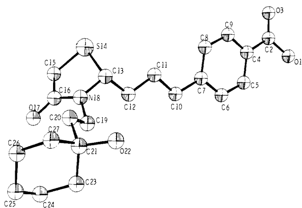
Figure 1. A perspective drawing of (+)- 5b showing the conformation in the solid state as well as the absolute configuration. Hydrogens have been omitted for clarity.
