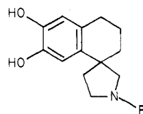
7, R = H, Me
