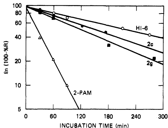
Figure 2. Semilogarithmic plot of \ln(100 - \% \text{ reactivation}) vs. incubation time for reaction of ethyl methylphosphonyl-AChE with 10 \mu\text{M} of compounds 2c, 2g, 2-PAM, and HI-6.
