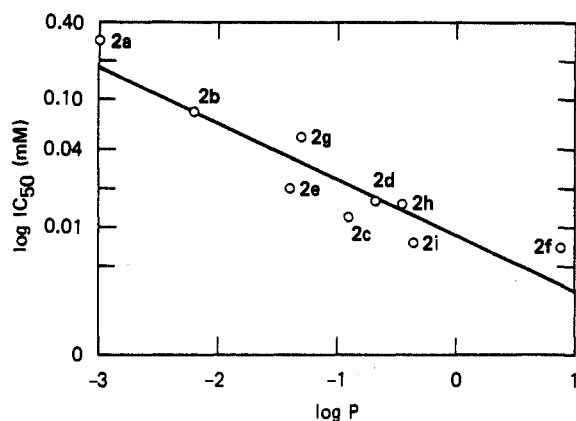
Figure 1. AChE inhibition potency ( \log IC_{50} ) vs. octanol:water partition coefficient ( \log P ) for type 2 compounds.
