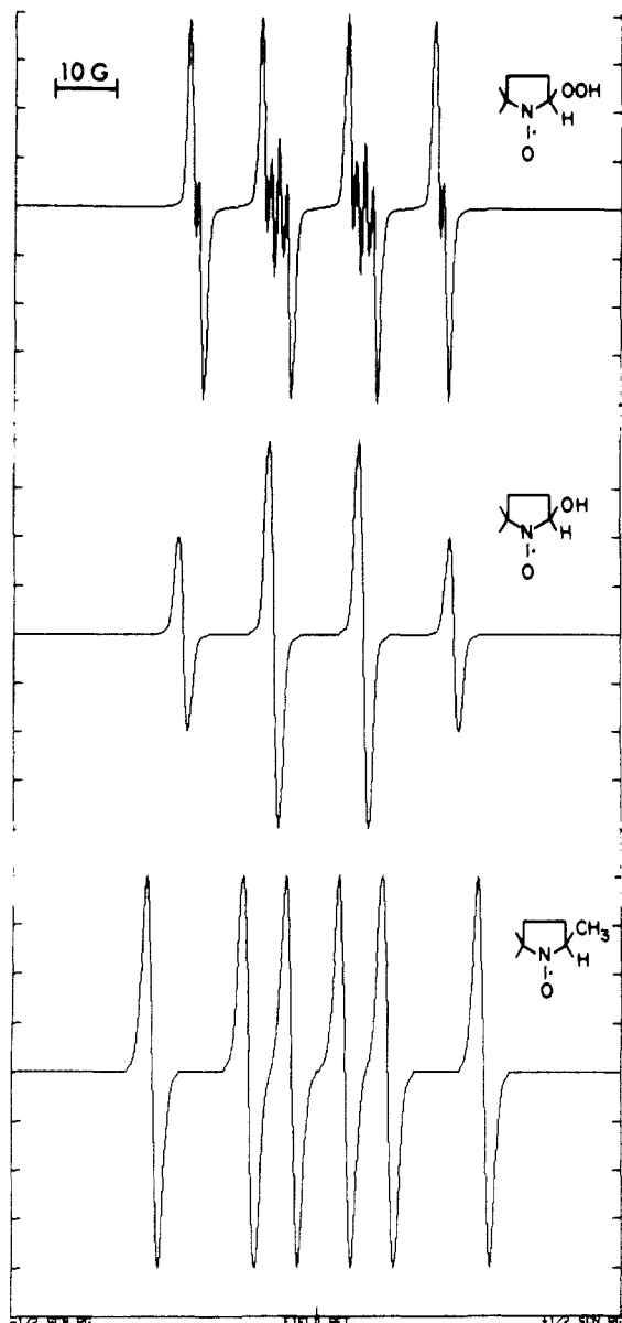
Figure 2. Computer simulation of ESR spectra for 2,2-dimethyl-5-hydroxy-1-pyrrolidinyloxy (DMPO-OH) and 2,2,5-trimethyl-1-pyrrolidinyloxy (DMPO-CH 3 ). The hyperfine splittings are as follows: for DMPO-OOH, A_N = 14.3 G, A^{H_2} = 11.7 G, and A^{H_1} = 1.25 G; for DMPO-OH, A_N = A_H = 14.87 G; for DMPO-CH 3 , A_N = 15.31 and A_H = 22.00 G.
