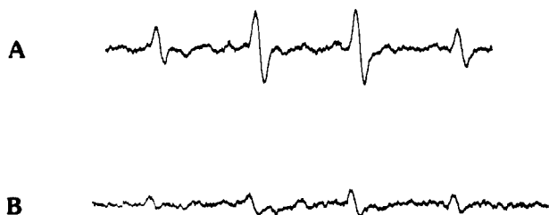
Figure 1. ESR spectra obtained when enterocytes were incubated with DMPO in the presence (A) and absence (B) of menadione (0.1 mM in 0.14 M \text{Me}_2\text{SO} ). The ESR spectrum in A is characteristic of DMPO-OH. Microwave power was 20 mW; the modulation frequency was 100 kHz with an amplitude of 1 G. Sweep time was 12.5 G/min and the receiver gain was 8 \times 10^3 with a response time of 1 s; A_H = A_N = 14.9 G.
