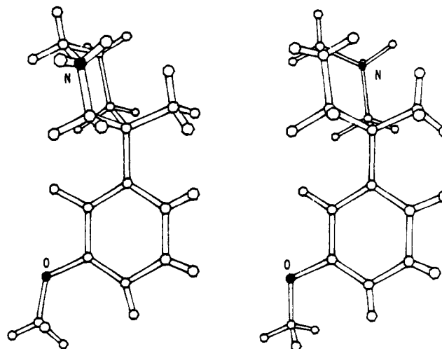
Figure 1. Molecular structure from X-ray determination of (–)-D-tartrate salt of the resolved (+)-5 analogue 3-methyl-3-( m -methoxyphenyl)piperidine, and its simulated enantiomer in proposed antagonist orientations. The drawing shows the correct absolute configuration of the molecule based on the known configuration (–)-D-tartrate salt acid. The interring torsion angle J(C_2C_1C_7C_8) = 62.8^\circ .
