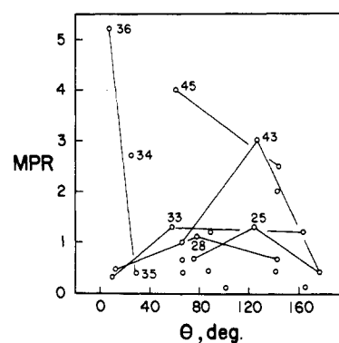
Figure 4. Relationship between coronary vasoactivity, as MPR vs. adenosine, and the direction of aryl dipole moment, \theta , among the N^6 -(arylethyl)adenosines. Solid lines join data from positional isomers, one member of which is designated by number in Table V. See text for additional discussion.
