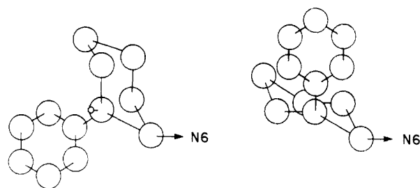
Figure 3. N 6 substituent of N 6 -[(1 R ,2 S )- trans -2-phenylcyclohexyl]adenosine, 20 , showing the two chair conformations that constitute extremes of the pseudorotational cycle of the cyclohexane moiety. Note how interconversion between the two conformations markedly changes the position of the phenyl moiety. Studies of molecular models of analogues 16-20 show that the phenyl group of the conformer shown at the left occupies a volume of space inaccessible to the phenyl groups of 16-19 .
