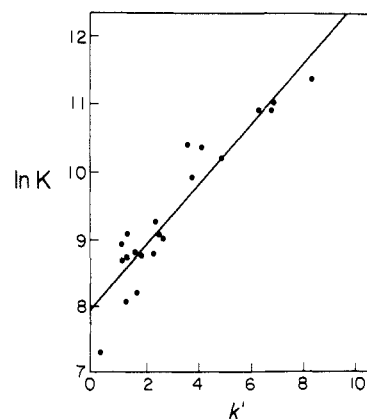
Figure 2. Influence of the hydrophobicity of the N 6 substituent on the binding of N 6 -phenyl- and N 6 -alkyladenosines to bovine serum albumin. The dissociation constant of the analogue-albumin complex, K , serves as a measure of binding affinity and k' , which is related to the retention time of the analogue on a reverse-phase HPLC column, is an index of hydrophobicity. The least-squares linear regression equation describing the relationship between K and k' is \ln K = 7.96 \pm 0.15 + 0.45 \pm 0.039k' , r^2 = 0.87 .
