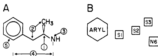
Figure 1. Hypothetical model of the N 6 region of the dog coronary artery A2 adenosine receptor. (A) Structure of the C-6 substituent of 1 showing chemical features that could be determinants of coronary vasoactivity, namely: (1) absolute configuration at the propyl C-2 chiral center, (2) the size and hydrophobicity of propyl C-1 and C-3, (3) the chemistry of N 6 , particularly its potential for hydrogen bonding, (4) the length of the alkyl chain separating the phenyl group from N 6 , and (5) the chemical attributes of the phenyl group. A previous report 13 examines factors 1–3, the present report concerns factors 4 and 5. (B) Topography of the N 6 region, depicted as consisting of aryl, S-1, S-2, S-3, and N-6 subregions complementary to the structure of the N 6 substituent of 1.
