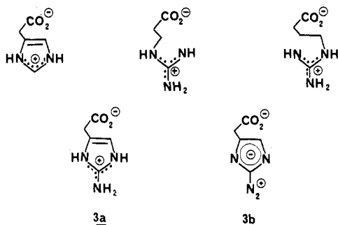
Chart I. Chemical Structures of Imidazoleacetic Acid, 2-Aminoimidazole-4(5)-acetic Acid ( 3a ), 2-Diazoimidazole-4(5)-acetic Acid ( 3b ), Guanidinopropionic Acid, and Guanidinobutyric Acid
