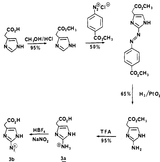
Scheme I. Syntheses of 2-Aminoimidazole-4(5)-acetic Acid ( 3a ) and the Corresponding Diazonium Salt 3b
