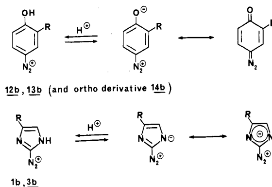
Scheme II. Diazonium-Diazo Equilibrium Derived from o - and p -Aminophenols and 2-Aminoimidazoles
