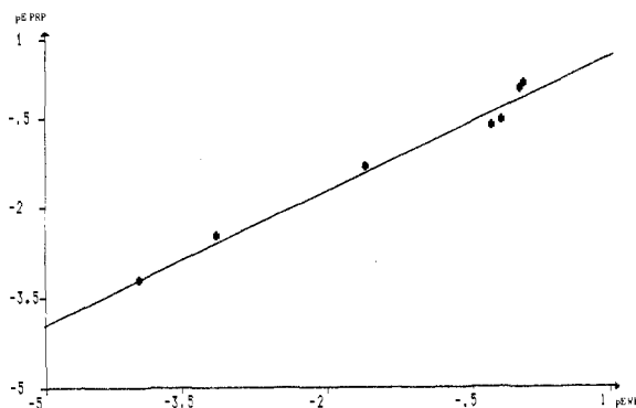
Figure 2. Relationship between pE PRP = -log (EC 50 PRP) and pE WP = -log (EC 50 WP) for compounds Ia-Ig. The regression equation is pE PRP = -0.156 (±0.195) + 0.773 (±0.098) pE WP. n = 7, s = 0.199, r = 0.989, F (1,5) = 238.98.
