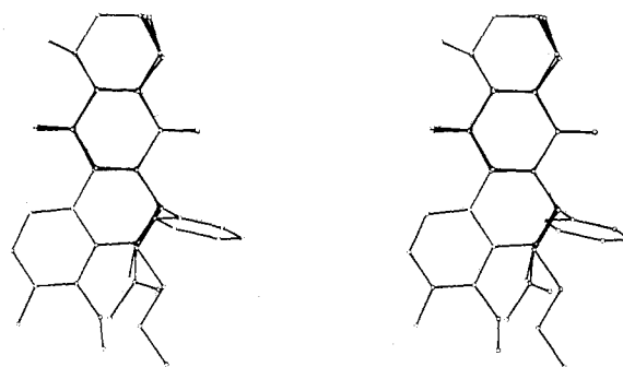
Figure 4. Superimposed structures of primin (2), ( R )-3,4-dimethoxydalbergione (3), deoxylapachol (4), and cyripedin (5).
