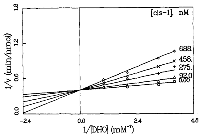
Figure 1. Double-reciprocal plot of dihydroorotase activity at variable concentrations of dihydro-L-oroate (0.25, 0.3, 0.5, 1.0 mM) and at changing fixed levels of ( \pm )- cis -1 (0, 92.0, 275.0, 458.0, and 688.0 nM) in 0.167 M Tris-HCl (pH 8.5)–1 mM dithiothreitol. The initial velocities are in units of nanomoles of N -carbamoyl-aspartate/minute. The lines drawn through the experimental points (the average of triplicate determinations) were obtained from fitting of the data to eq 1. Other experimental conditions are described in the Experimental Section.
