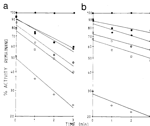
Figure 4. Alternate method for plotting time- and concentration-dependent inhibition by thiol androgens. a: 3 ; b: 2 . Concentrations are the same as in Figure 3.
