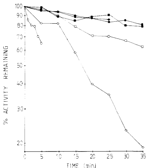
Figure 5. Paraoxon protection experiments: ●, no inhibition; ○, 0.5 \mu\text{M} 2; ◆, 2.0 \mu\text{M} 7 + paraoxon; ◇, 2.0 \mu\text{M} 7; ■, 0.5 \mu\text{M} 8 + paraoxon; □, 0.5 \mu\text{M} 8.
