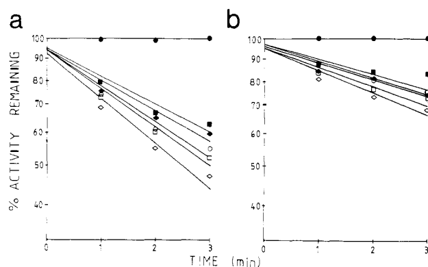
Figure 3. Time- and concentration-dependent loss of aromatase activity by thiol androgens: (a) ●, 0.0; ■, 40; ◆, 60; ○, 100; □, 167; ◇, 500 nM 10 \beta -mercaptoandrost-4-ene-3,17-dione ( 3 ). (b) ●, 0.0; ■, 35; ◆, 50; ○, 75; □, 100; ◇, 500 nM 19-mercaptoandrost-4-ene-3,17-dione ( 2 ).
