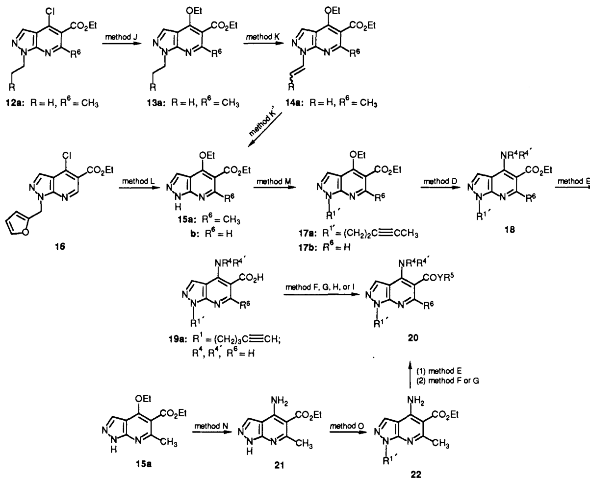
Scheme II a,b
