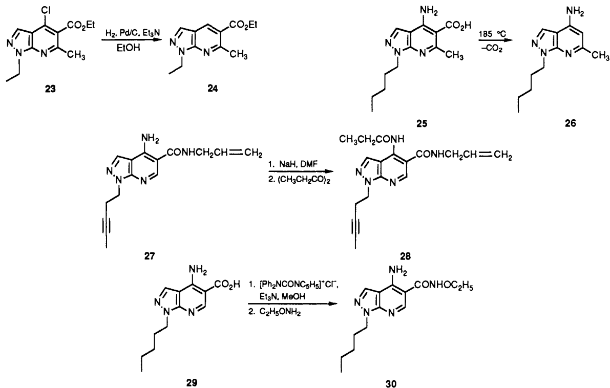
Scheme IV
