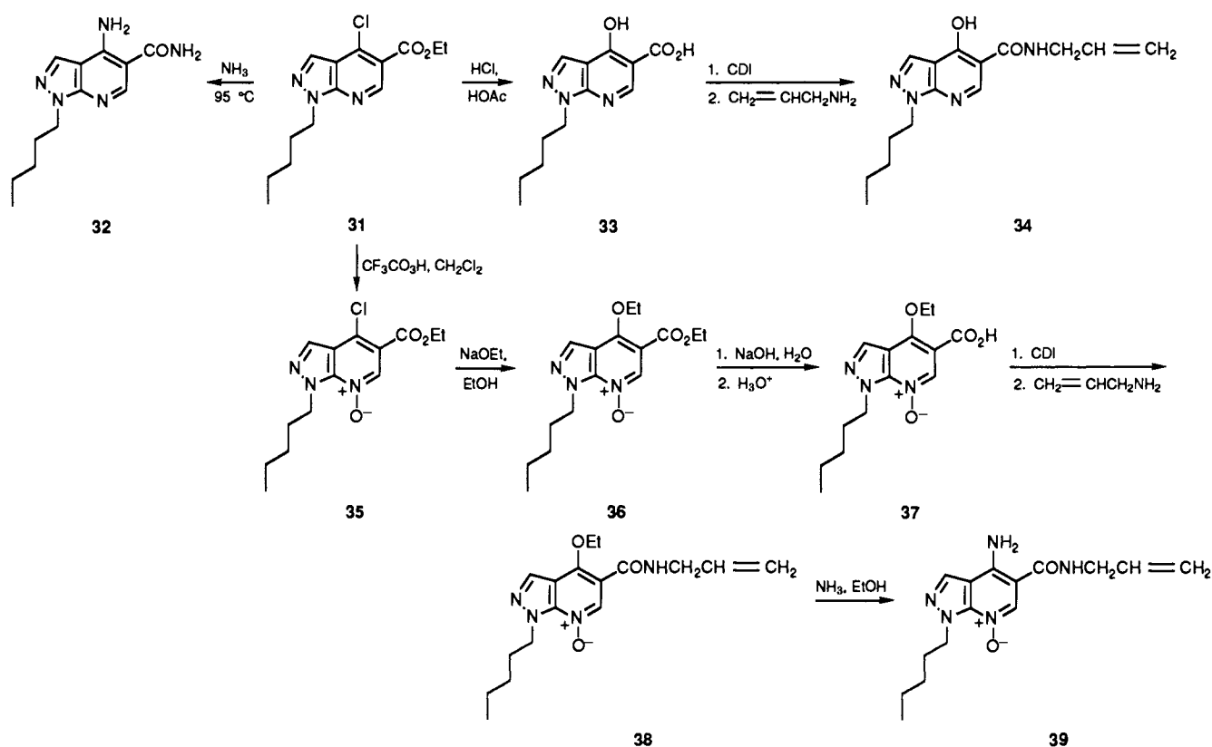
Scheme IV
