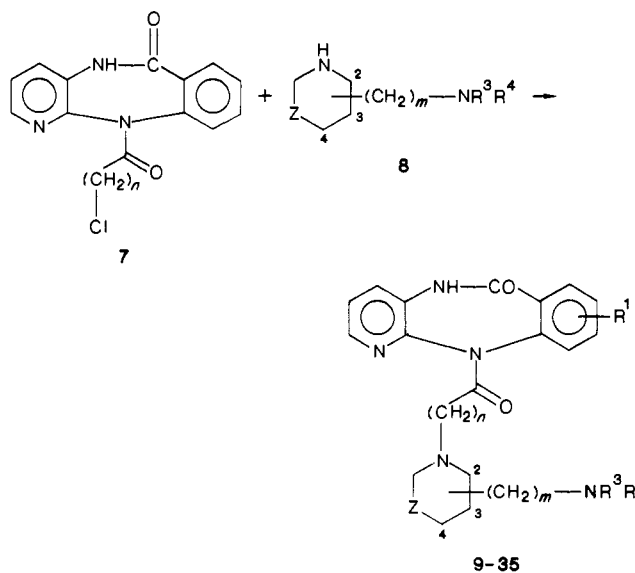
Figure 2. Structural variations within the side chain and the pyridobenzotricyclic of AF-DX 116: Z = bond, CH 2 , (CH 2 ) 2 ; n = 0, 1, 2; m = 1, 2; R 1 = H, 8-Cl, 8-CH 3 , 8-C 2 H 5 , 9-Cl, 9-CH 3 .
