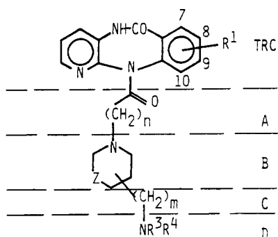
Structural variations of side chains and pyridobenzotricyclic of AF-DX 116.
