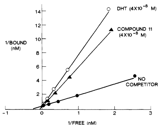
Figure 1. Lineweaver-Burk analysis demonstrating competitive inhibition of [ 3 H]dihydrotestosterone (DHT) binding to rat ABP by DHT and compound 11. The binding of 2.5 nM [ 3 H]DHT to rat epididymal cytosol was determined at 4 °C for 2 h in the absence (no competitor) and presence of a constant concentration of unlabeled competitor (indicated in parentheses). Each data point represents the mean of two determinations.
