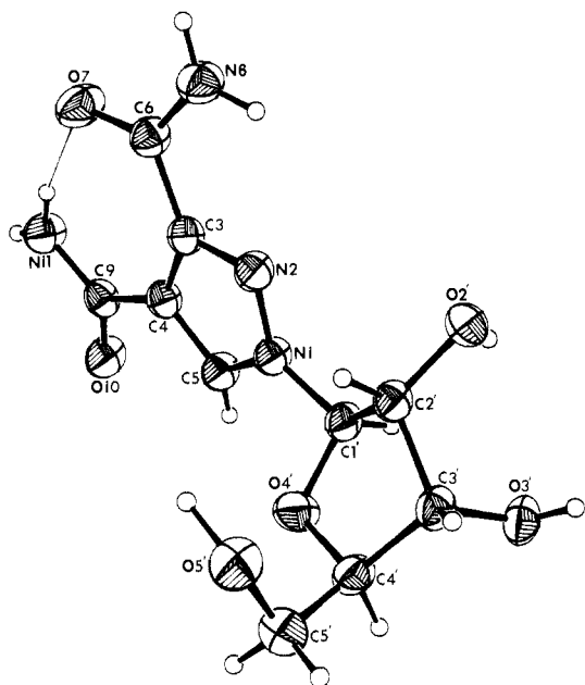
Figure 2. ORTEPII drawing of compound 3.
