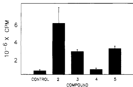
Figure 4. Chemiluminescence of reduced luminol measured in cultures of HL-60 cells following treatment with compounds and stimulation with phorbol ester. Cells were incubated in growth medium alone (control) or with 30 \mu M compound 2, 60 \mu M compound 3, 40 \mu M compound 4, or 60 \mu M compound 5 for 4 days at 37 ^{\circ} C. Chemiluminescence was stimulated with tetradecanoylphorbol ester as described in the Experimental Section. The intensity of chemiluminescence (cpm) varies with time (cf. Figure 5). The maximum values of the intensity of chemiluminescence are shown here. The values shown are the mean and standard deviation for triplicate determinations in one experiment which is representative of three separate experiments that gave identical results.
