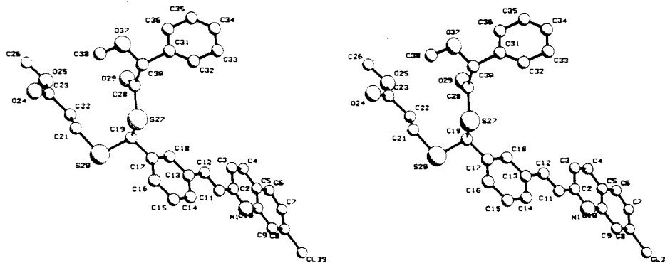
Figure 1. A computer-generated stereodrawing of 5 showing the atom labeling. Hydrogen atoms are eliminated for clarity.
