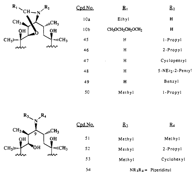
Scheme V. Structures of 9- N,N -Dialkyl Derivatives of Erythromyclamine
