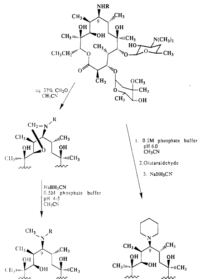
Scheme IV. Synthesis of 9- N,N -Dialkyl Derivatives of Erythromyclamine
