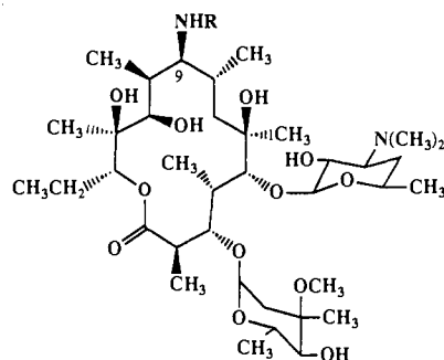
Scheme III. Structures of 9- N -Alkyl Derivatives of Erythromyclamine
