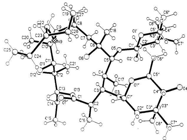
Figure 1. X-ray structure of 9- N -(2-ethyl-1-butyl)erythromyclamine (18).
