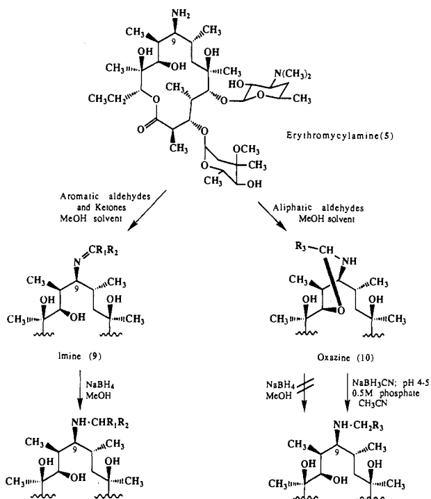
Scheme II. Synthesis of 9- N -Alkyl Derivatives of Erythromyclamine
