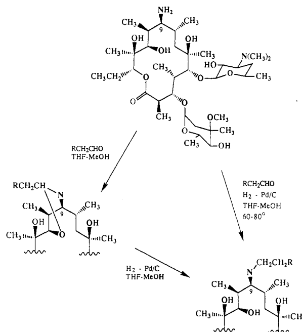
Scheme VI. Alternative Synthesis of 9- N -Alkyl Derivatives of Erythromyclamine
