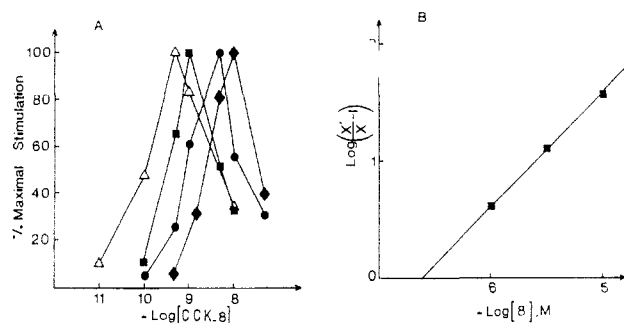
Figure 1. Effects of compound 8 on CCK 8 -induced amylase release from guinea pig pancreatic acini: (A) amylase release of CCK 8 was measured alone ( \Delta ) or in the presence of compound 8, ( \blacksquare ) 10^{-6} M, ( \bullet ) 3 \times 10^{-6} M, and ( \blacklozenge ) 10^{-5} M; (B) Schild plot of the antagonism by compound 8 [ \log x'/x - 1 = 0.96 \log B + 6.37 ( r = 0.998 ), pA_2 = 6.63 ]. Points represent the mean of three experiments each performed in duplicate.
