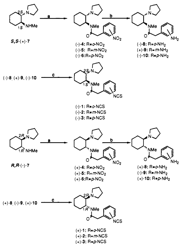
Scheme I. Synthesis of Aryl Isothiocyanate Derivatives of (1 S ,2 S )- and (1 R ,2 R )-U50,488 a
