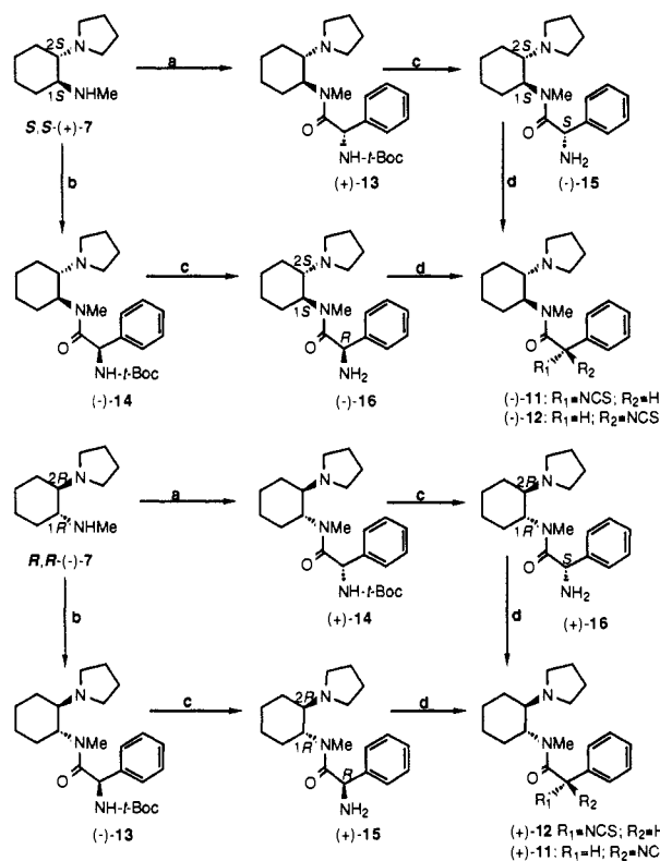
Scheme II. Synthesis of Alkyl Isothiocyanate Derivatives of (1 S ,2 S )-U50,488 and (1 R ,2 R )-U50,488 a
