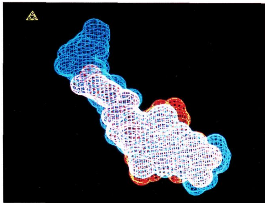
Figure 2. Overlay of the volume maps of active compounds (blue) and inactive compounds (red).
