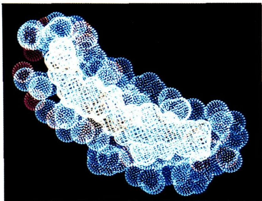
Figure 5. The compound binding site in HRV-14 highlighted by van der Waals surfaces with compound 3 inserted.
