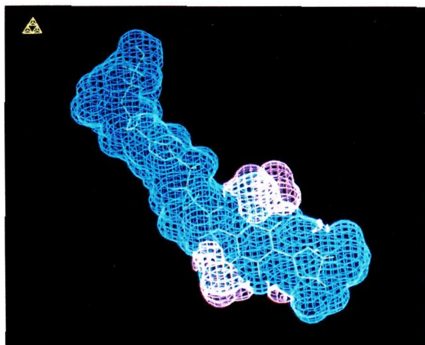
Figure 4. Difference between the inactive (red) and active (blue) volume maps (Boolean "minus") showing the space occupied by active compounds with compound 1 inserted.
