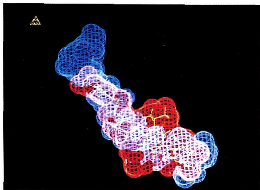
Figure 3. Boolean "minus" displaying the volume occupied by the inactive compounds in red with compound 12 inserted.
