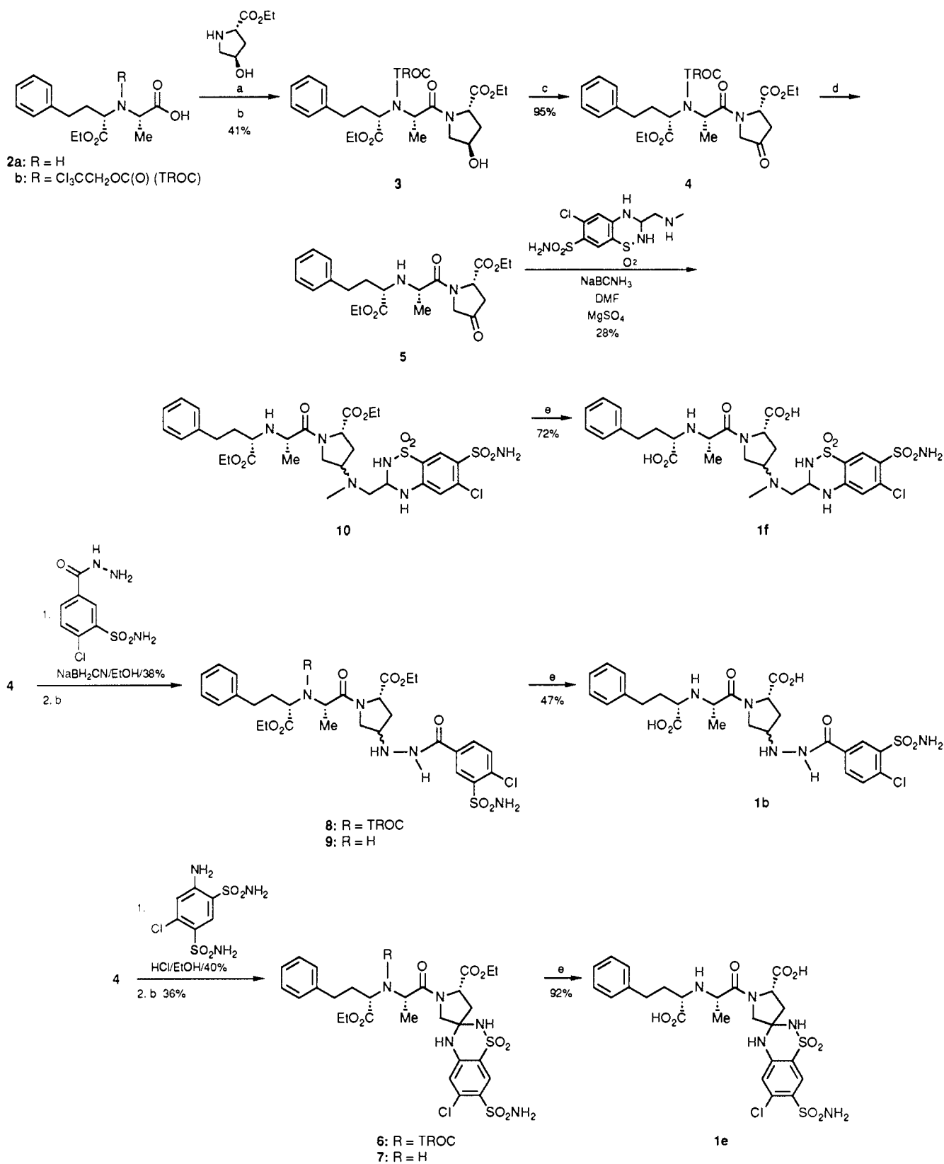
Scheme I a
