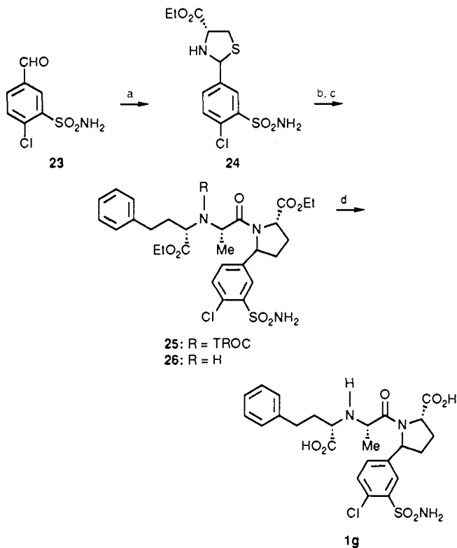
Scheme IV a
