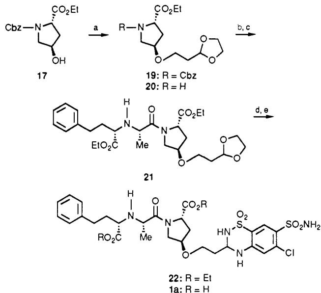
Scheme III a
