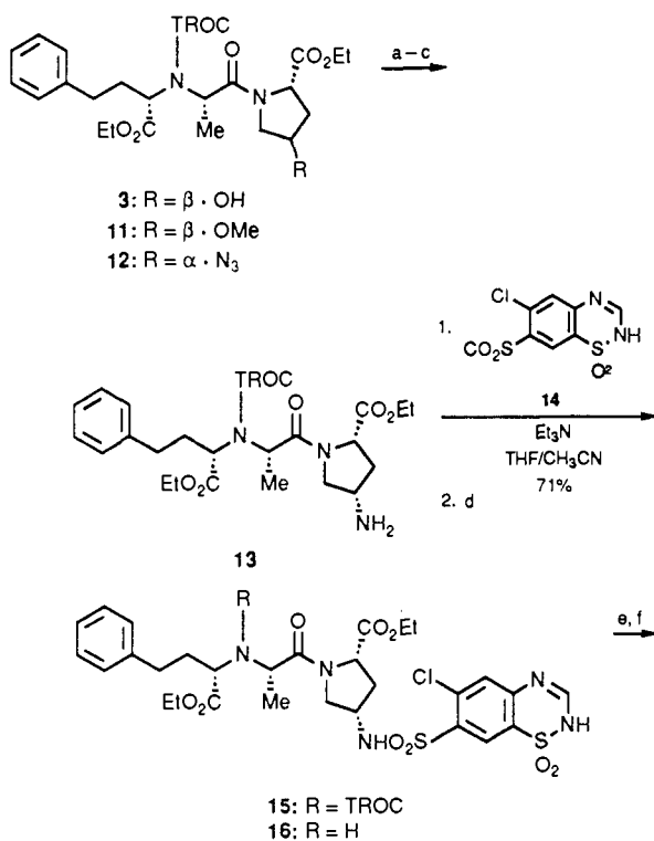
Scheme II a
