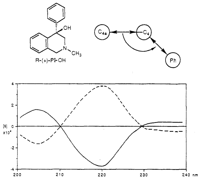
Figure 1. CD spectra of R -(+)- and S -(-)-1 in methanol (0.0103 mg/mL). Each spectrum was the result of four computer averaged scans: (—) R -(+)-1; (---) S -(-)-1.
