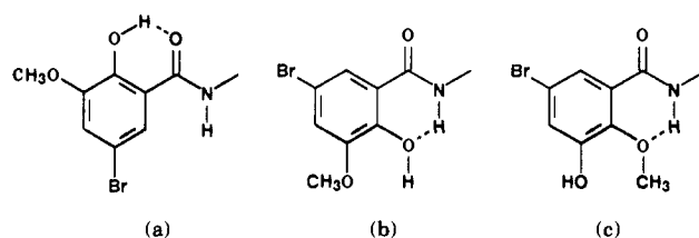
Figure 1. Two possible hydrogen bonded rotamers (a) and (b) of salicylamide 12 shown in relation to the 1000-fold more active regioisomer 8 (c).
