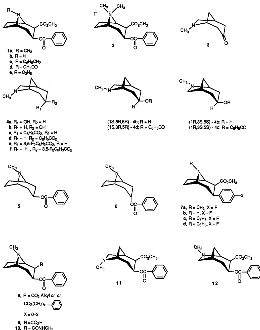
Figure 1. Structural formulas for cocaine and analogues. Structures with wedged bonds are optically active.
