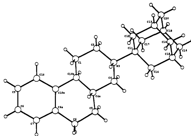
Figure 1. Computer-generated drawing of 27 showing its stereochemistry.
