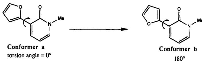
Chart IX. Heat of Formation Curves by the AM1 Method for the Rotation about the Central Bond (a-b-c-d) in Model Compounds
