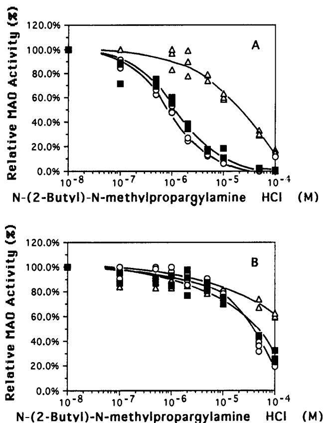
Figure 1. Stereospecific effect of N -(2-butyl)- N -methylpropargylamine hydrochloride on MAO activities. The inhibitory activity of the R -(-)-18 [O] and S -(+)-19 [Δ] enantiomers as well as the racemic mixture 3 [■] on rat liver mitochondrial MAO activities toward MAO-B substrate 2-phenylethylamine ( 1.9 \times 10^{-5} M) [panel A] and MAO-A substrate 5-hydroxytryptamine ( 5 \times 10^{-4} M) [panel B] were estimated as described in the Experimental Section. Results are for triplicate determinations.
