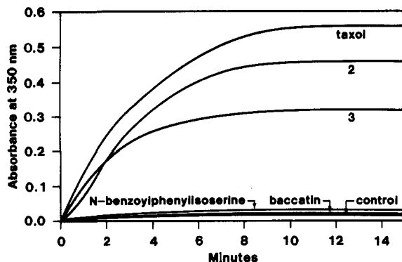
Figure 2. Tubulin at 10 \mu\text{M} was polymerized at 37 ^{\circ}\text{C} in the presence of 5 \mu\text{M} taxol or its derivatives and 0.5 mM GTP in PEM buffer. The increase in turbidity was monitored by the apparent absorbance at 350 nm.
