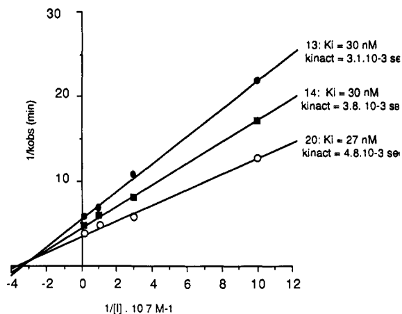
Figure 2. Double-reciprocal plots of the observed pseudo-first-order rate constants of inactivation ( k_{obs} ) versus inhibitor concentration for 13 (●), 14 (■), and 20 (○).
