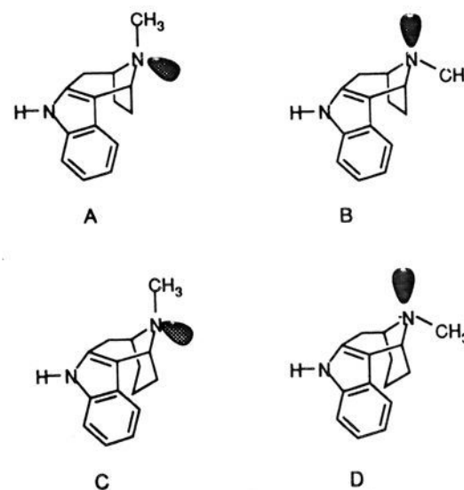
Figure 1. Invertomers of ethylene- and propylene-bridged \gamma -carbolines.
