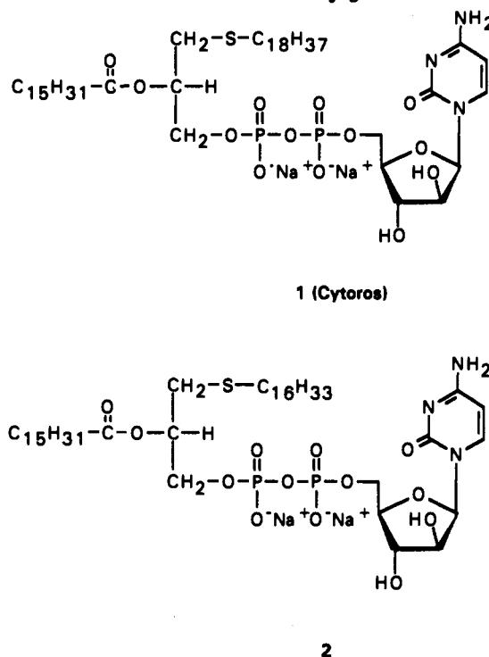
Chart I. Chemical Structure of Conjugates 1 and 2
