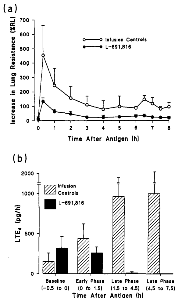
Figure 3. IV infusion of 44 at 8 µg/kg/min in allergic sheep ( n = 4 ): (a) effect on postantigen bronchoconstriction and (b) effect on postantigen urinary LTE 4 excretion.
