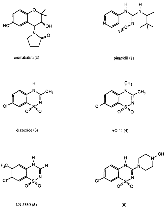
Figure 1. Chemical structure of different potassium channel openers (1-3) and of diazoxide analogues reported to exhibit an hyperglycemic activity (4-6).
