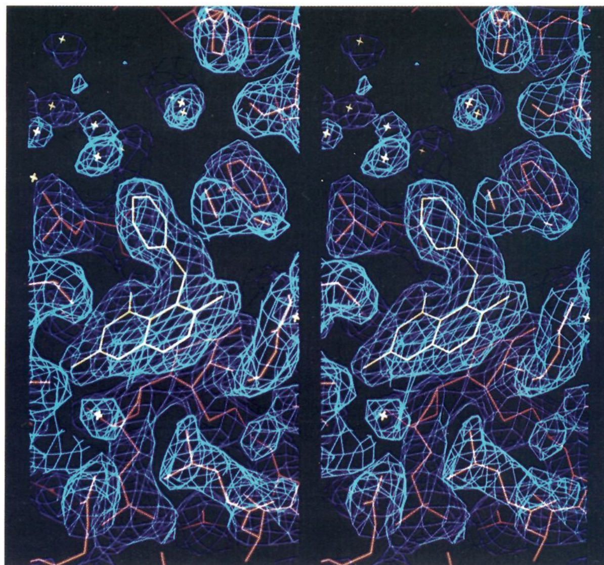
Figure 2. Stereoview of the electron density map of the crystal structure of compound 8 complexed with E. coli TS and 5-FdUMP at 2.5-Å resolution computed with coefficients 2F_{\text{obs}} - 2F_{\text{calc}} and phases calculated after 18 cycles of refinement for which the R factor was 17.8%.
