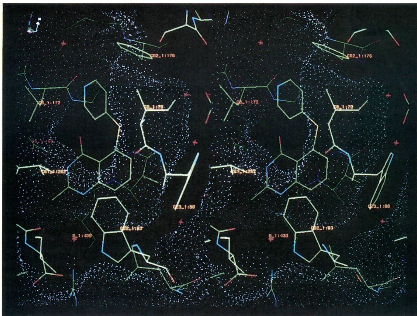
Figure 1. Stereoview of the ternary X-ray structure of compound 6, E. coli TS, and 5-FdUMP. The protein and ligand atoms are displayed in green (carbon), red (oxygen), blue (nitrogen), and yellow (sulfur). The water molecules are displayed as red crosses, and the solvent accessible surface of the protein is highlighted in light blue. Ile79, Trp80, Trp83, Asp169, Leu 172, Phe176, Val262, and H 2 O 430 are labeled.
