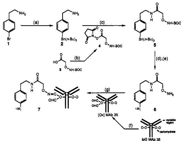
Figure 1. Phenethylamine iodination scheme. (a) [(n\text{-Bu})_3\text{Sn}]_2 , \text{Pd}[(\text{C}_6\text{H}_5)_3\text{P}]_4 , toluene, 95^\circ\text{C} ; (b) \text{NHS} , \text{DCC} , \text{Et}_3\text{N} , \text{EtOAc} ; (c) \text{4} , \text{Et}_3\text{N} , \text{EtOAc} ; (d) (i) \text{Na}^{[125]\text{I}}\text{I} , \text{MeOH-H}_2\text{O} ; (ii) chloramine-T; (iii) \text{Na}_2\text{S}_2\text{O}_5 ; (e) 90% aqueous \text{TFA} ; (f) \text{NaIO}_4 , \text{PBS} ( \text{pH} 6); (g) [\text{Ox}]\text{Mab} 35, 0.15 M \text{HOAc}/\text{NaOAc} ( \text{pH} 4).
