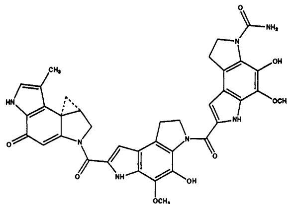
(+)-CC-1065
