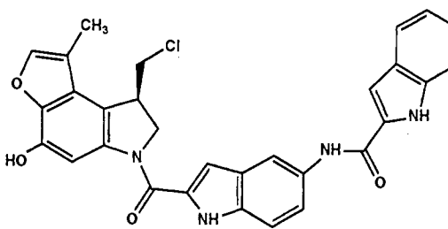
18 (LY297950)
