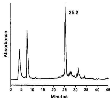
Figure 3. RP-HPLC elution profile of products following aminolysis of peptide-resin III. The elution gradient was 25–80% B in 40 min at a flow rate of 1.0 mL/min, where A was 0.1% TFA in H 2 O and B was 0.1% TFA in acetonitrile. Other conditions are given under Experimental Section. [Cys-(Acm) 2 ,Lys(Boc) 5 ,Thr( t Bu) 6 ,Cys(Acm) 7 ]octreotide eluted at 25.2 min.
