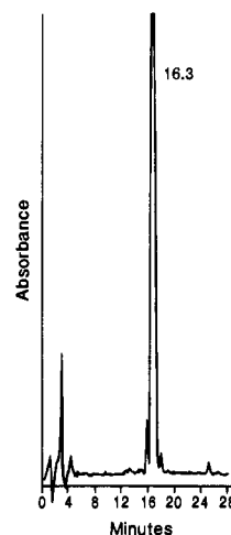
Figure 5. RP-HPLC elution profile of purified [D-Trp(Boc) 4 ,Lys(Boc) 5 ,Thr( t Bu) 6 ]octreotide. The elution gradient was 20–30% B in 40 min at a flow rate of 1.5 mL/min, where A was 0.1% TFA in H 2 O and B was 0.1% TFA in acetonitrile. Other conditions are given under Experimental Section. [D-Trp(Boc) 4 ,Lys(Boc) 5 ,Thr( t Bu) 6 ]octreotide eluted at 16.3 min.
