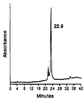
Figure 6. RP-HPLC elution profile of purified DTPA-D-Phe 1 -octreotide. The elution gradient was 10–60% B in 40 min at a flow rate of 1.0 mL/min, where A was 0.1% TFA in H 2 O and B was 0.1% TFA in acetonitrile. Other conditions are given under Experimental Section. DTPA-D-Phe 1 -octreotide eluted at 22.9 min.
