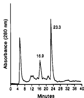
Figure 4. RP-HPLC elution profile of crude [D-Trp(Boc) 4 ,Lys(Boc) 5 ,Thr( t Bu) 6 ]octreotide. The elution gradient was 40–60% B in 40 min at a flow rate of 0.6 mL/min, where A was 0.1% TFA in H 2 O and B was 0.1% TFA in 2-propanol. Other conditions are given under Experimental Section. [D-Trp(Boc) 4 ,Lys(Boc) 5 ,Thr( t Bu) 6 ]octreotide eluted at 23.3 min.
