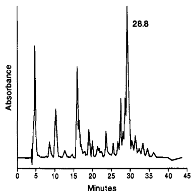
Figure 1. RP-HPLC elution profile of products following "mild" reductive cleavage of peptide-resin I. The elution gradient was 25–80% B in 40 min at a flow rate of 1.0 mL/min, where A was 0.1% TFA in H 2 O and B was 0.1% TFA in acetonitrile. Other conditions are given under Experimental Section. D-Phe-Cys(Acm)-Phe-D-Trp-Lys(Boc)-Thr( t Bu)-Cys-(Acm)-Thr(ol) eluted at 28.8 min.
